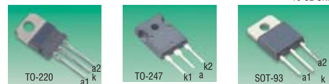
TO-220
